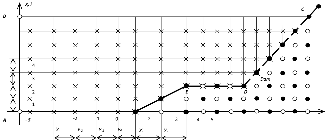
Fig.1. Finite difference grid for calculating the wave equation in the reservoir: • - points for determining velocities in the dam; o - points for determining stresses in the dam; X - points for calculating the potential F in the water storage.
